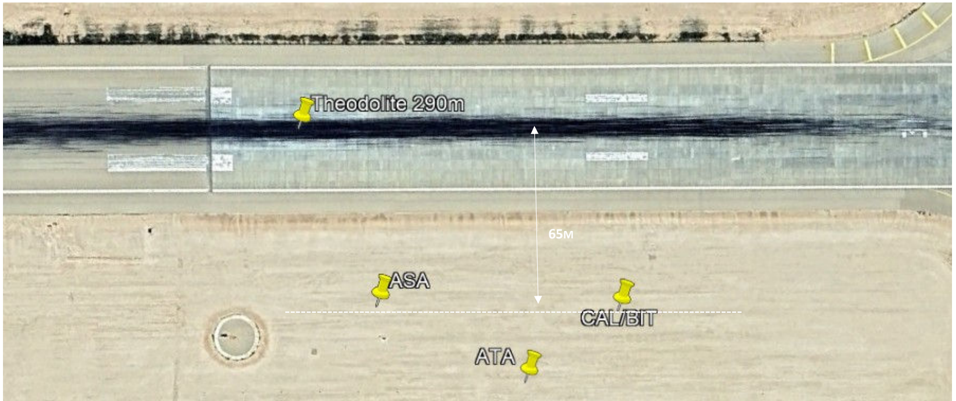
Figure 4 - Place cal/bit same distance from centerline as center of ASA beam , 65 meters is recommended
