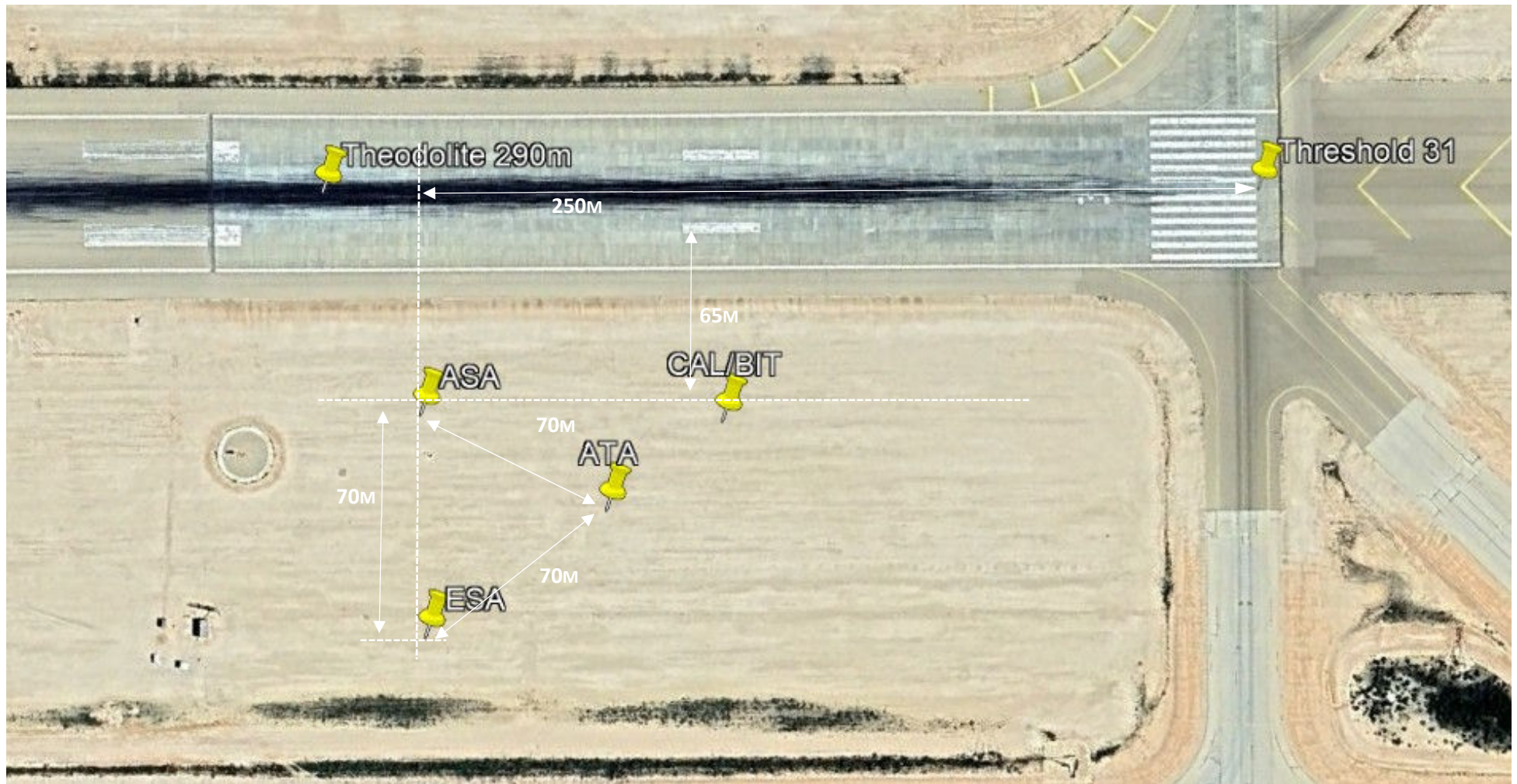
Figure 2 - Plan view detailed siting dimensions
